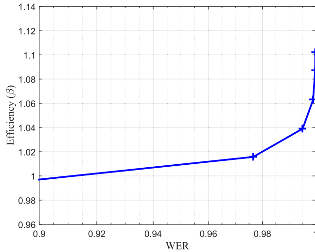
Figure 2. The values of \beta , equation (3), obtained for the length 10^5 rate 0.02, multi-edge LDPC code with degree distribution from [13] with a maximum of 5000 decoder iterations.
